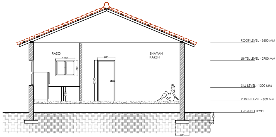
SECTION - BB'
